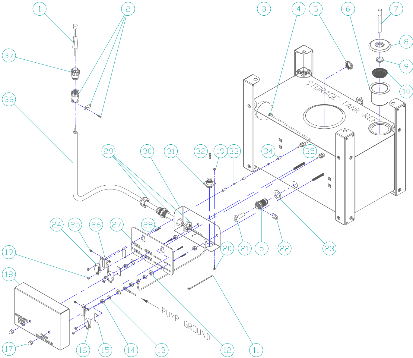
REAR RIGHT SIDE VIEW OF THE STORAGE TANK
