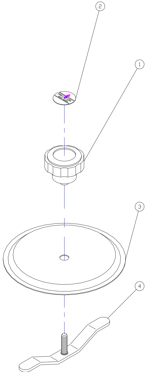
HOLDING TANK LID ASSEMBLY (PART # 500248)
