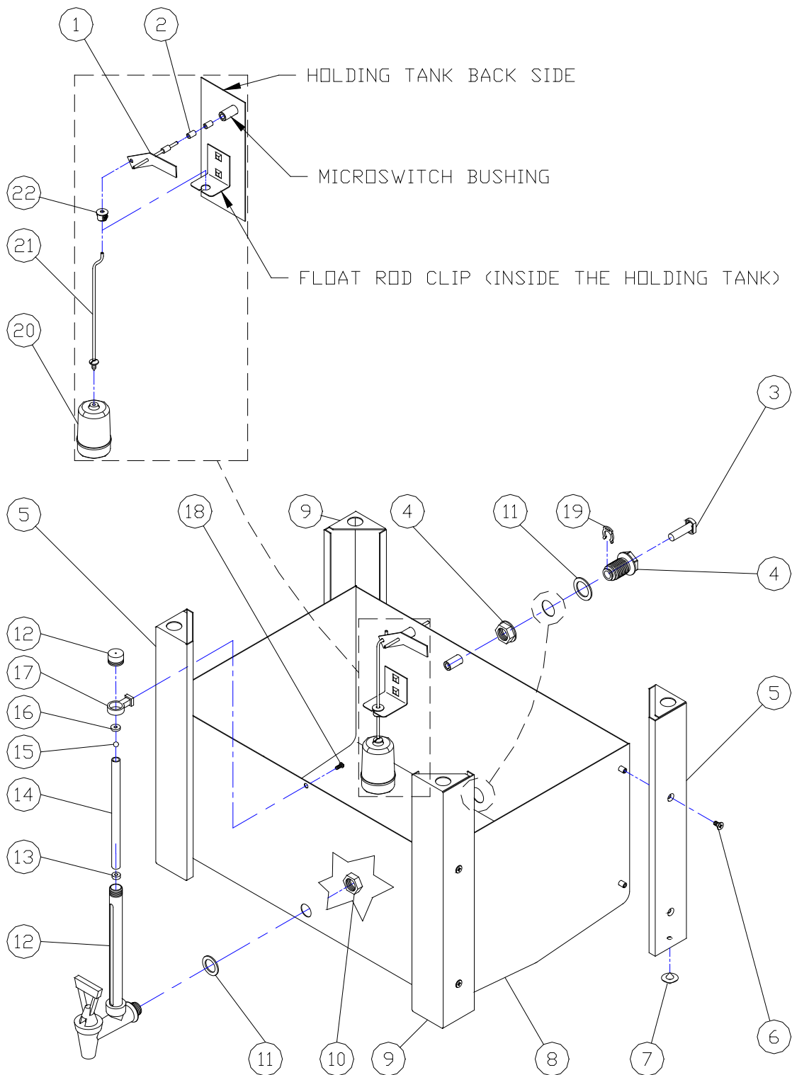
FRONT LEFT SIDE VIEW WITH TOP REMOVED
