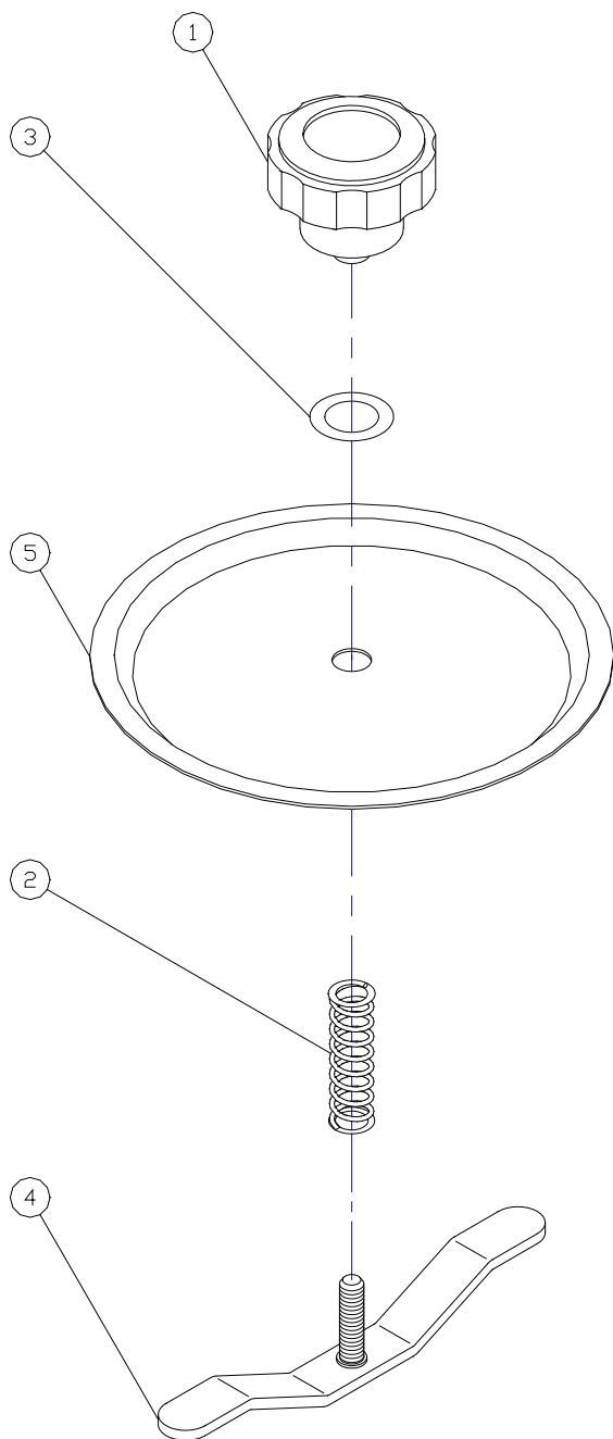
BOILING TANK LID ASSEMBLY (PART # 500319)
