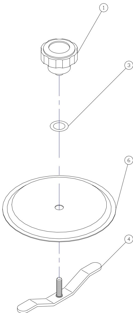
HOLDING TANK LID ASSEMBLY (PART # 500320)
