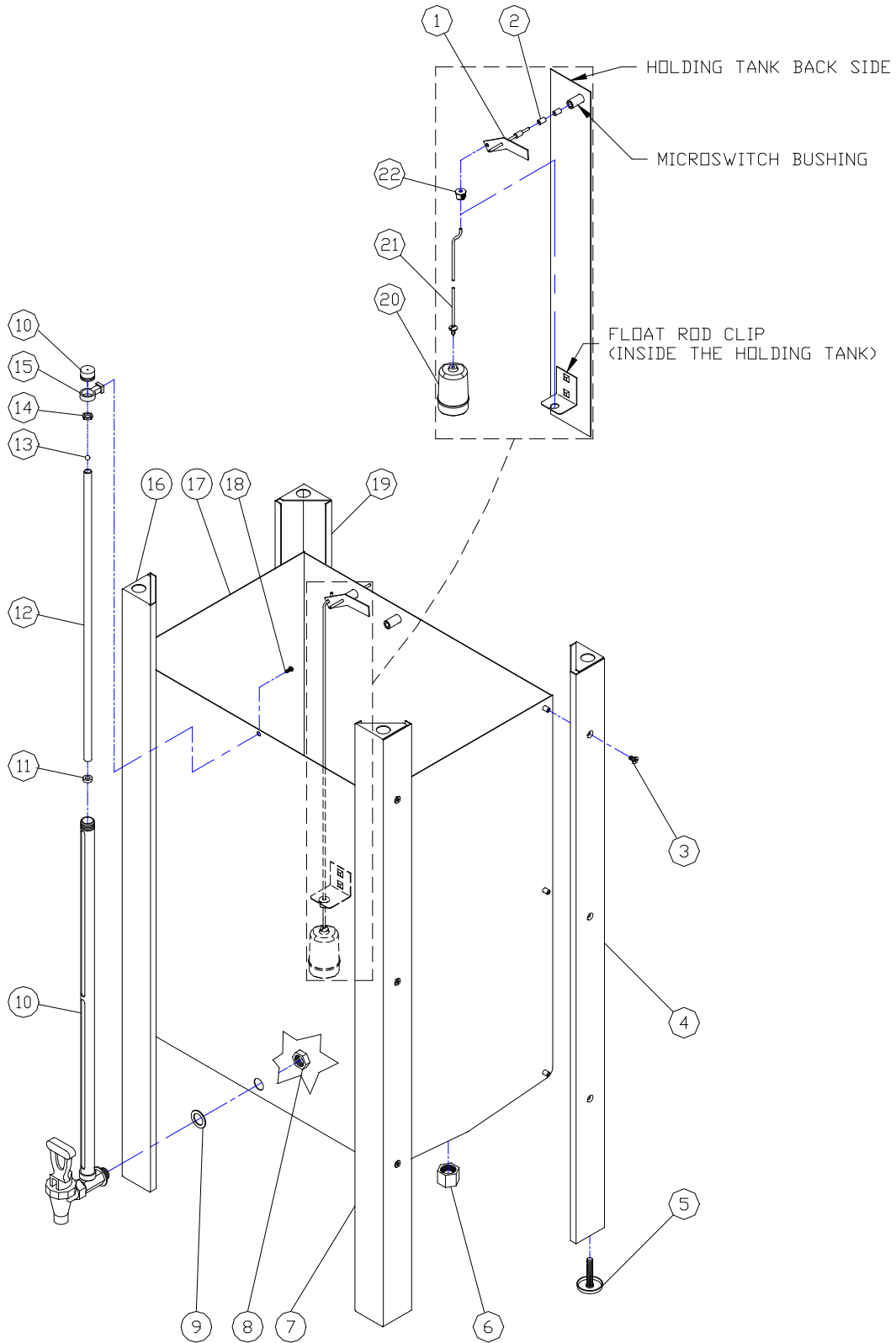
FRONT LEFT SIDE VIEW WITH TOP REMOVED
