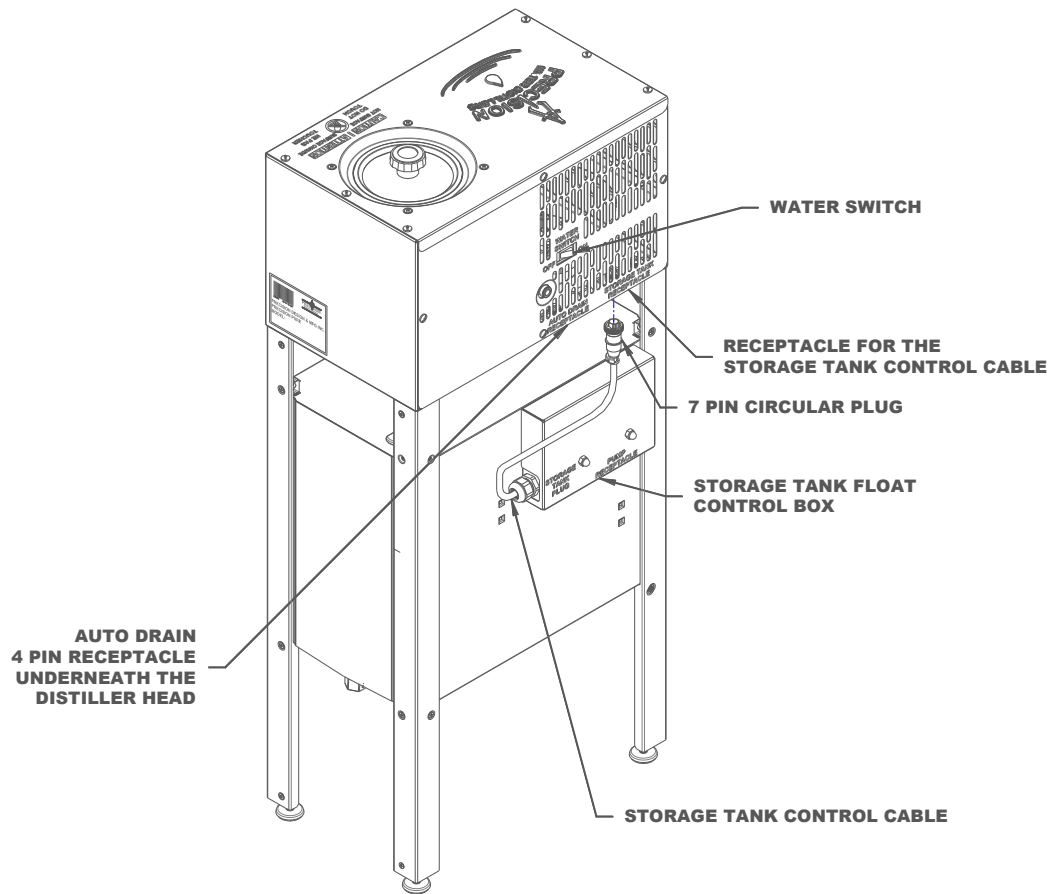
Electrical Connections-Rear View Diagram
