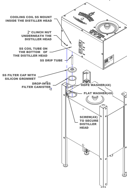
Water Distiller Head Removal Diagram
