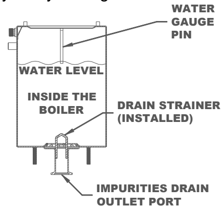
Boiling Tank Water Gauge Pin Diagram
