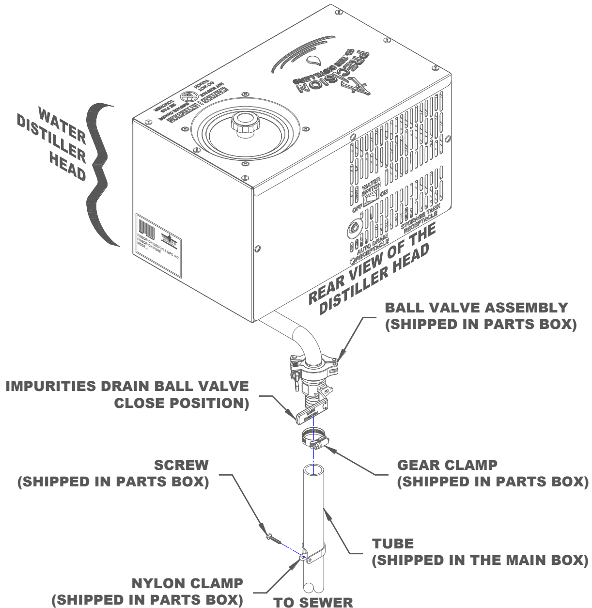
Manual Drain Valve Tube Installation Diagram
