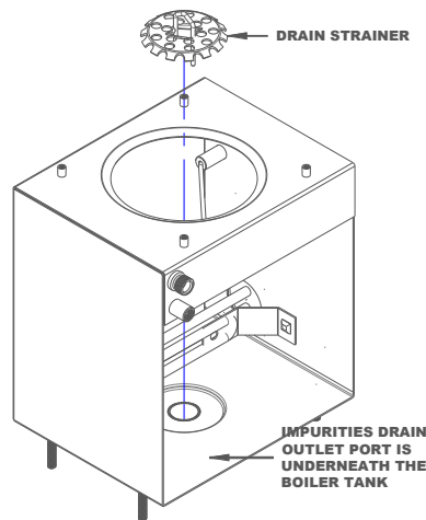
Boiling Tank Strainer Removal Diagram
