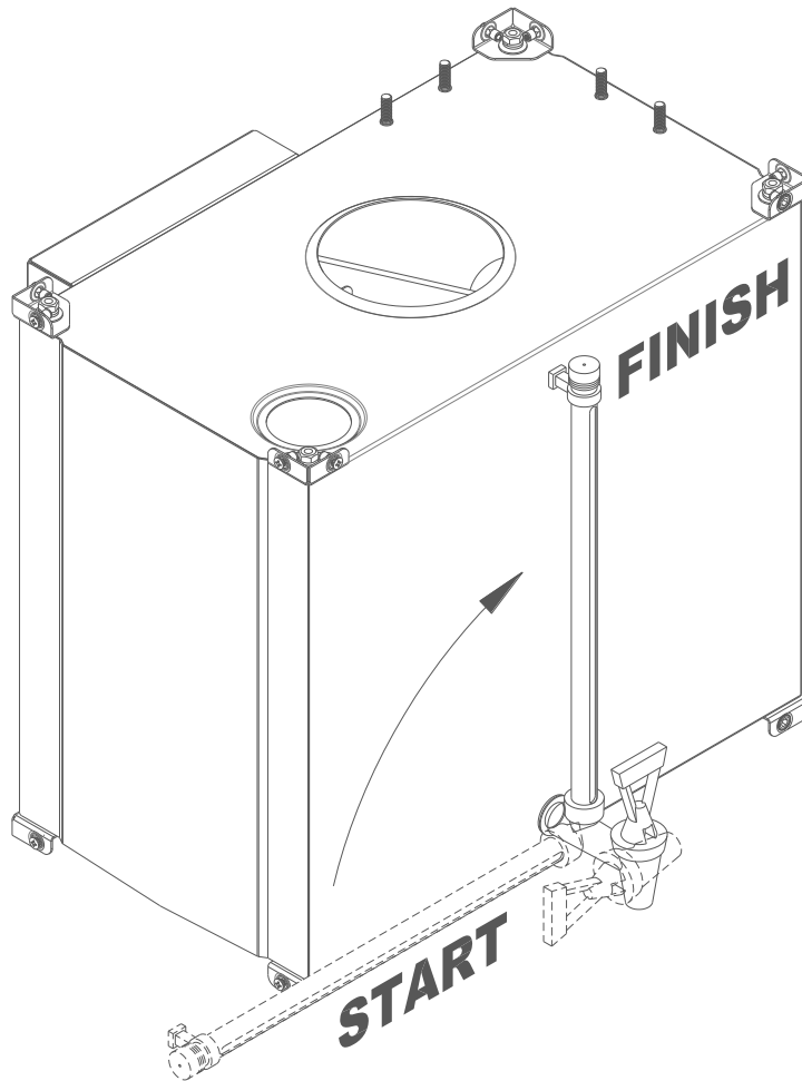
Tightening Sight Gauge Nut Diagram
