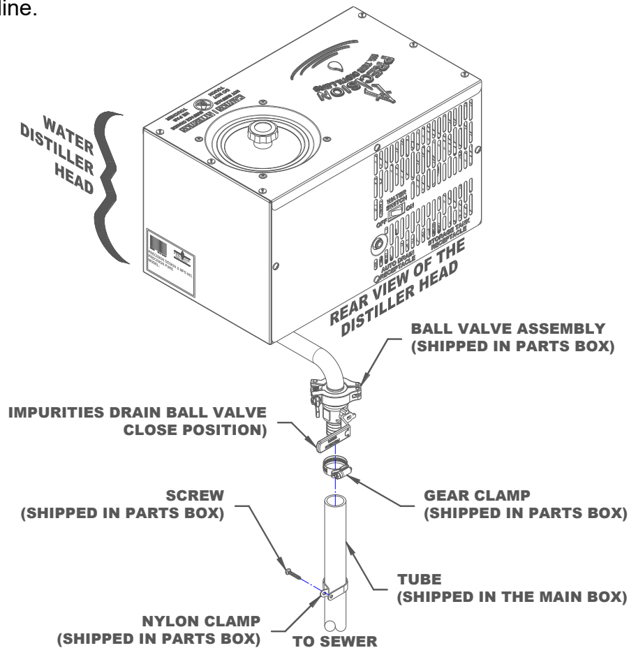
Drain Tube Removal Diagram
