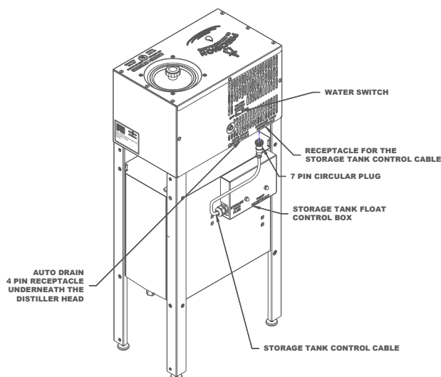
Control Cable Disconnect Diagram
