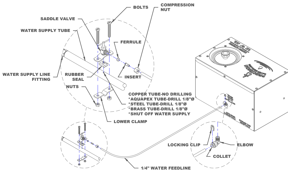
Feed Water Line Installation Diagram
