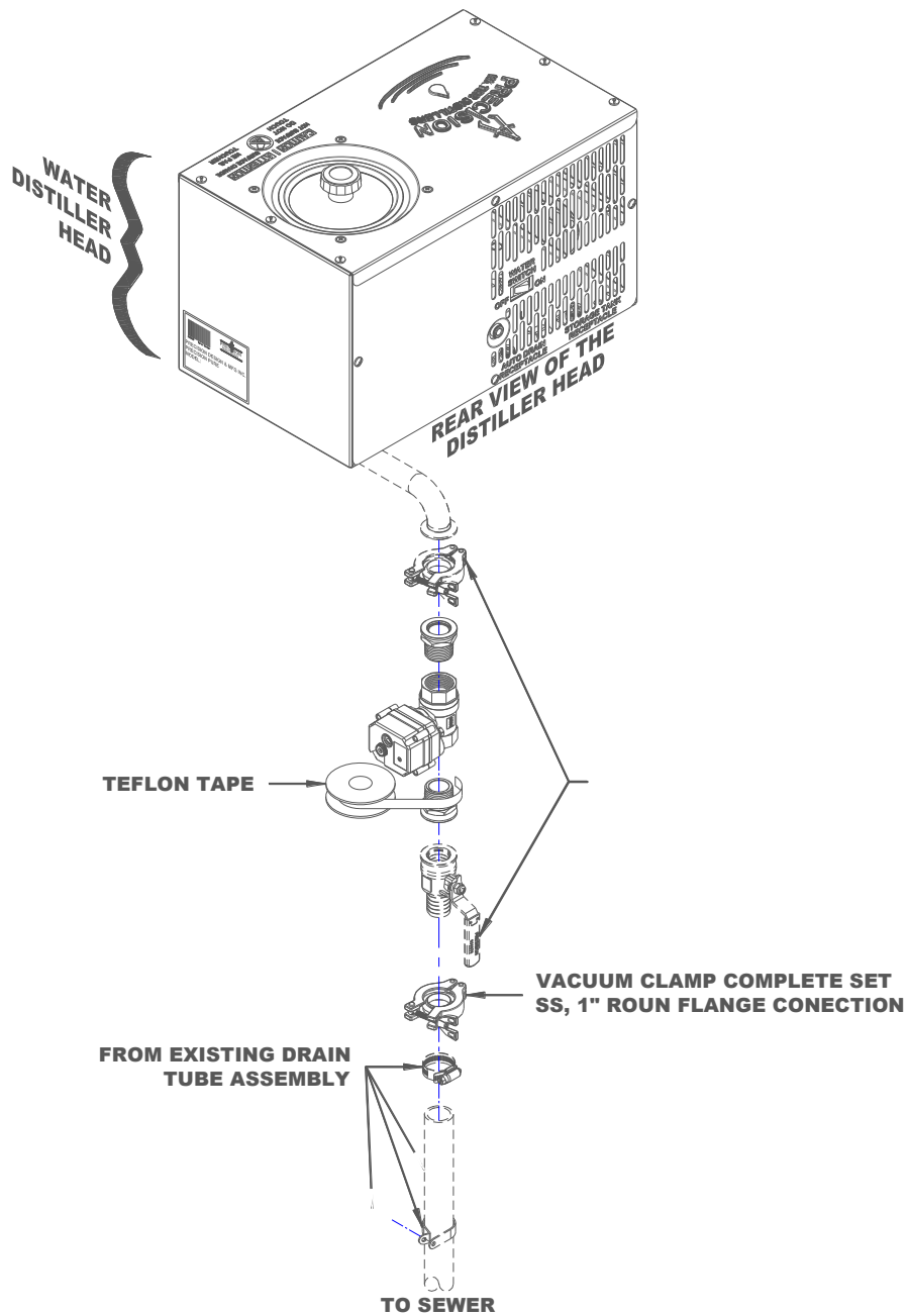
PWS AED-1 Plumbing Diagram
