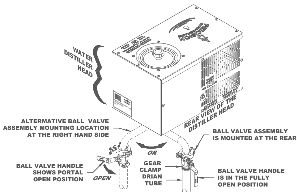
Manual Drain Valve Location Diagram
