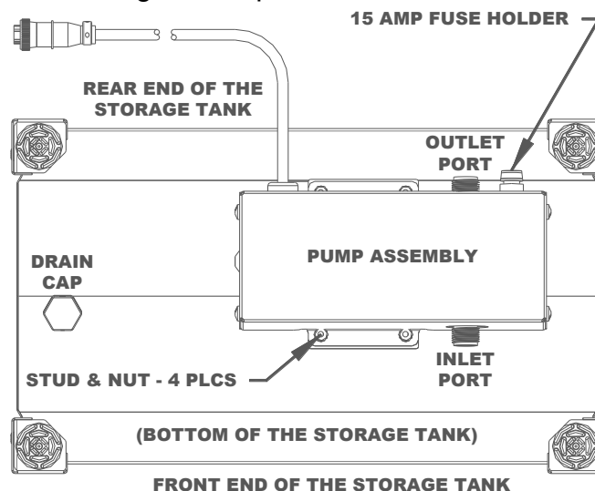
Automatic Pump Mounting Diagram
