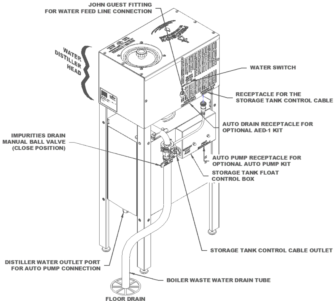
Water Distiller Box Components Diagram
