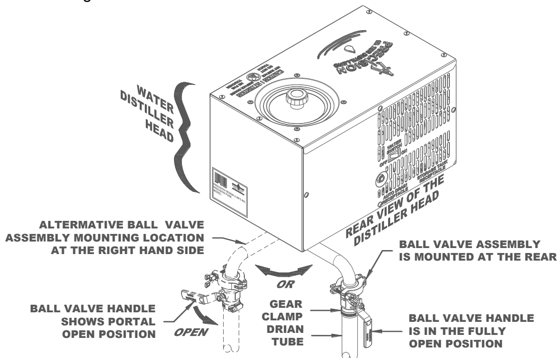
Manual Drain Valve Location Diagram
