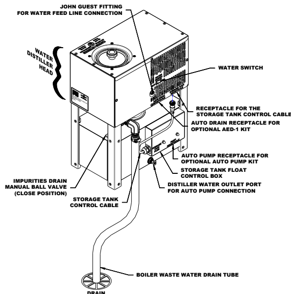
Electrical Connections-Rear View Diagram
