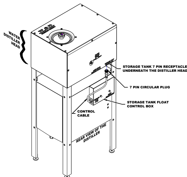
Control Cable Connection Diagram
