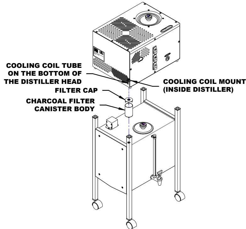
Charcoal Replacement Diagram
