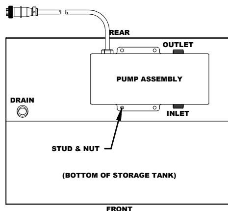
12-20 AUTOMATIC PUMP KIT - 1 DIAGRAM
