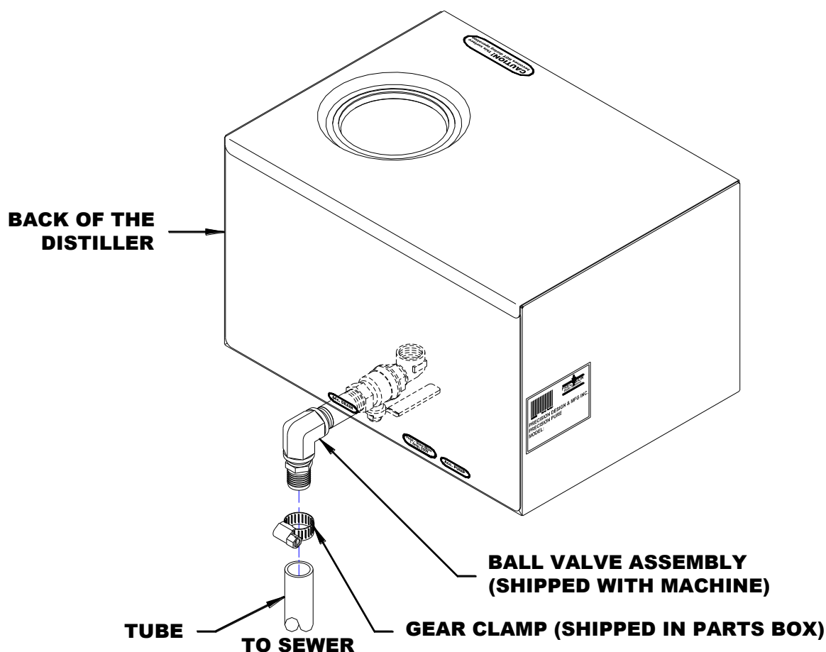
Manual Drain Valve Tube Installation Diagram
