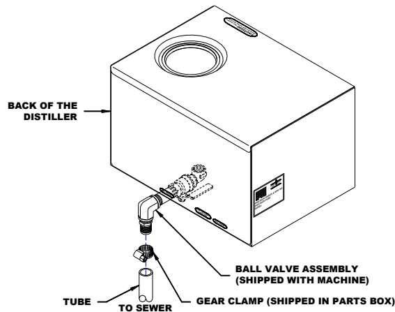
Boiling Tank Drain Valve Diagram
