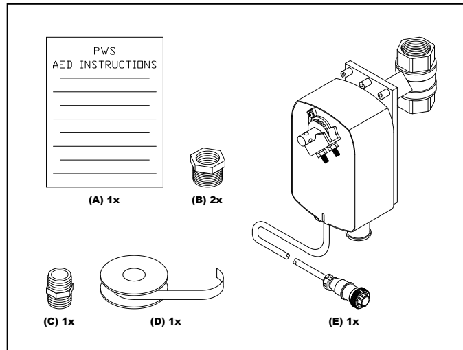
PWS-AED-1 Box Components Diagram PWS AED-1 Box Check Off List
