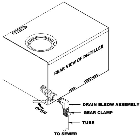
Manual Drain Valve Location Diagram
