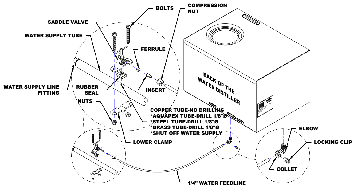
Feed Water Line Installation Diagram
