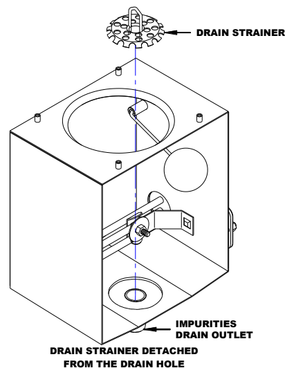
Boiling Tank Strainer Removal Diagram
