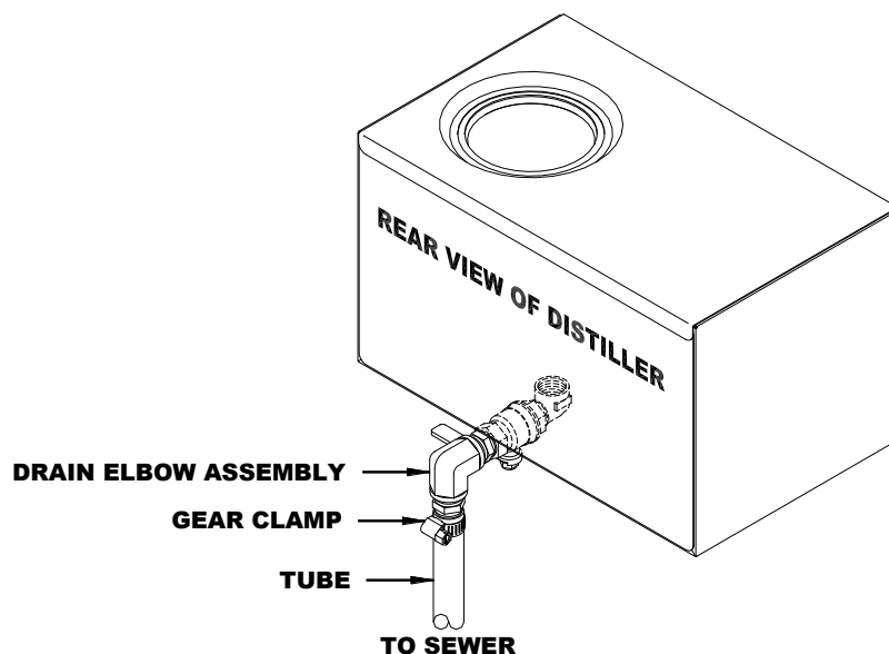
Manual Drain Valve Location Diagram
