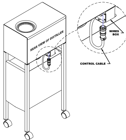
Control Cable Connection Diagram
