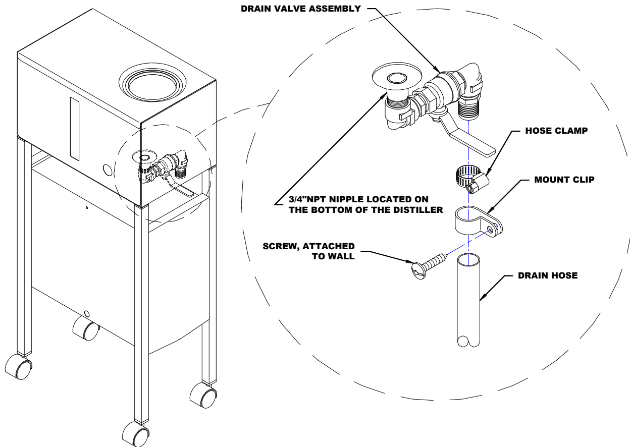
Water Distiller Wall Stabilizer Diagram
