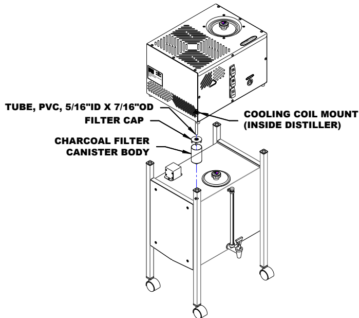
Water Distiller Head, Filter Canister and Storage Tank Steam Sterilization Diagram
