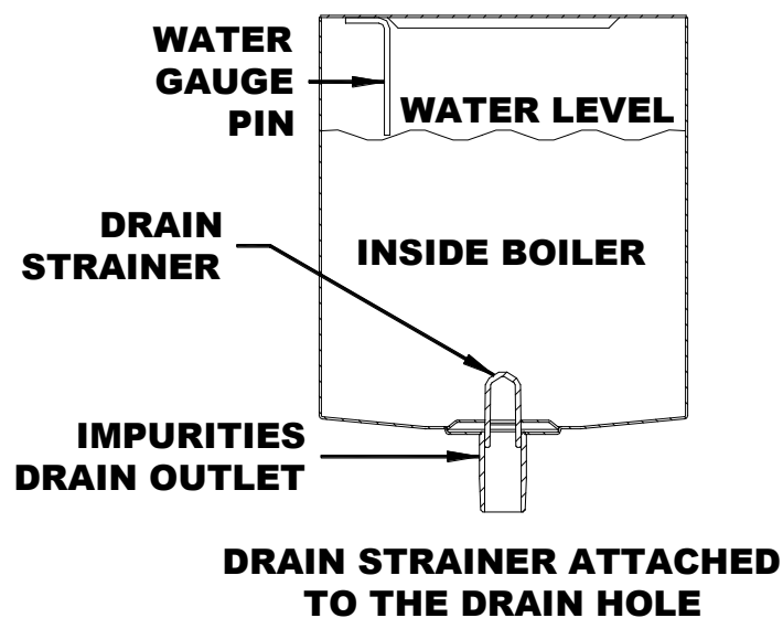
Boiling Tank Water Gauge Pin Diagram
