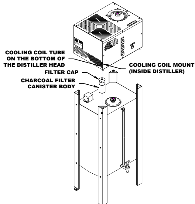
Water Distiller Head Removal Diagram
