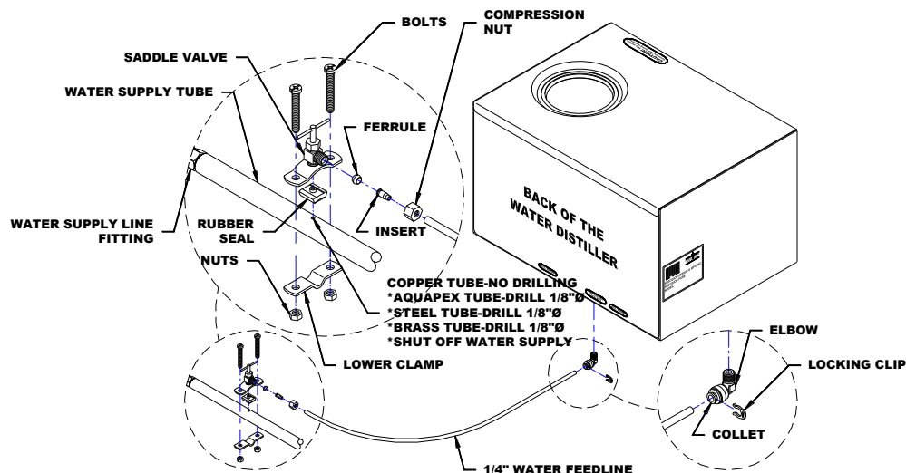
Feed Water Line Installation Diagram
