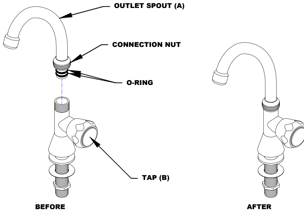
Pantry Faucet Assembly Diagram
