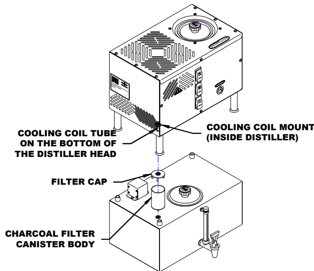
Charcoal Replacement Diagram
