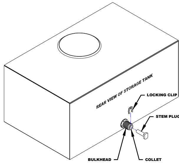
Bulkhead Stem Plug Removal Diagram
