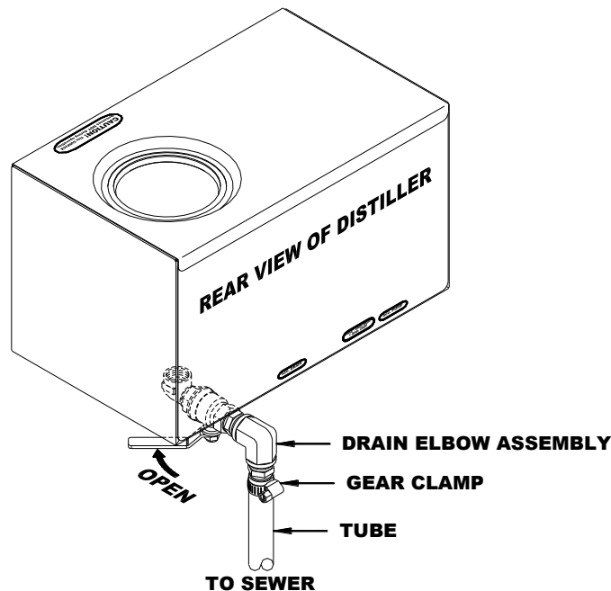
Manual Drain Valve Location Diagram
