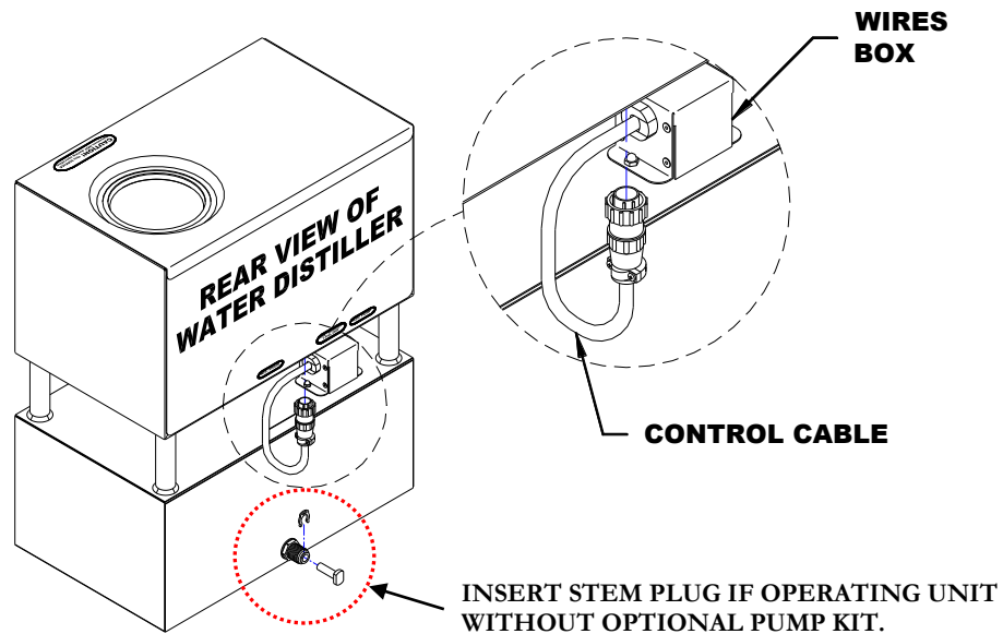
Control Cable Disconnect Diagram
