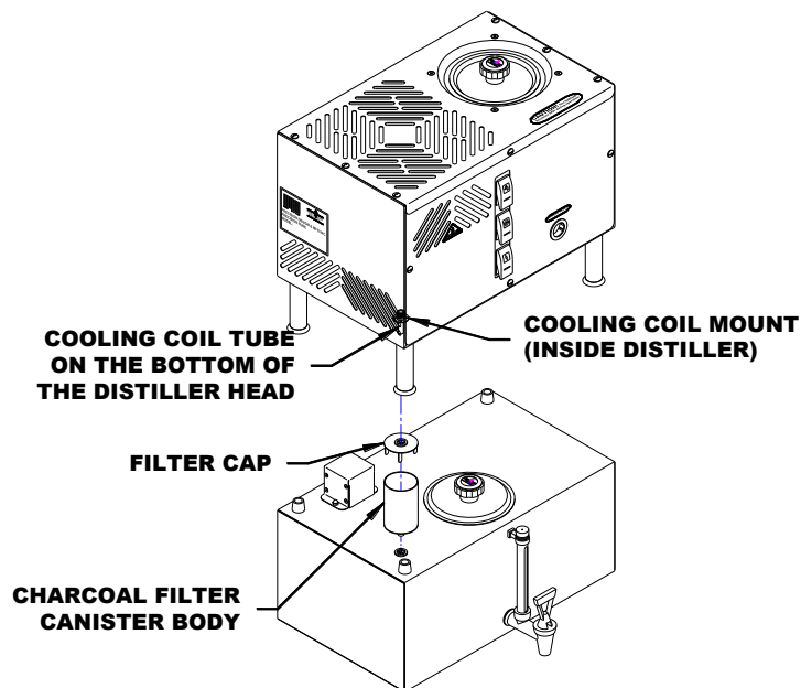
Water Distiller Head Removal Diagram
