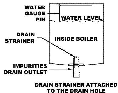
Boiling Tank Water Gauge Pin Diagram
