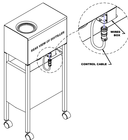
Control Cable Connection Diagram
