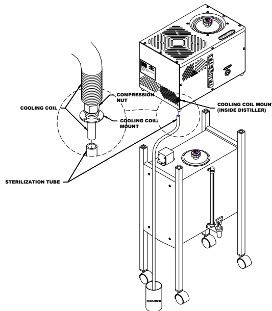
Water Distiller Head Steam Sterilization Diagram
