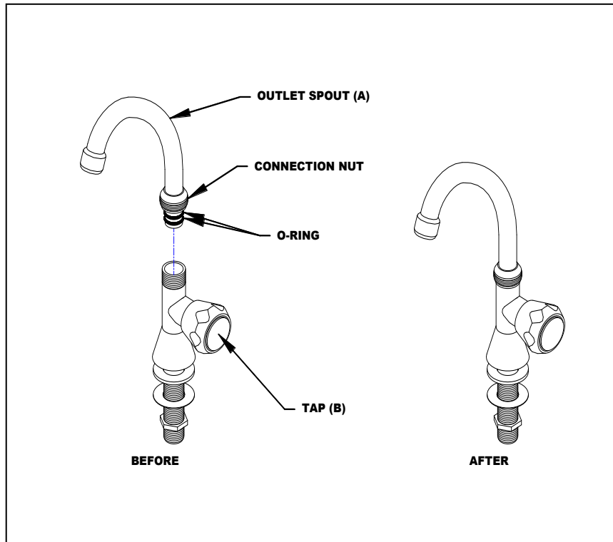
Pantry Faucet Assembly Diagram
