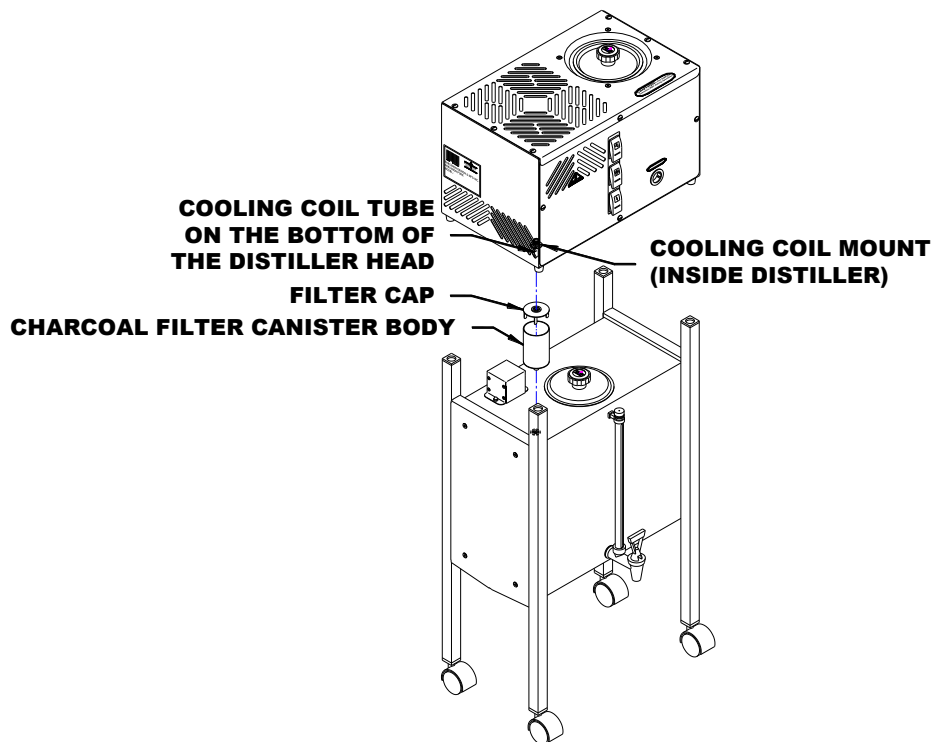
Water Distiller Head Removal Diagram
