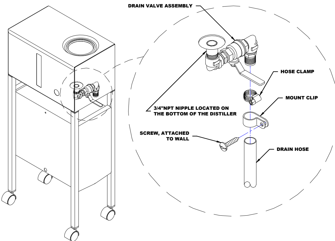
Water Distiller Wall Stabilizer Diagram
