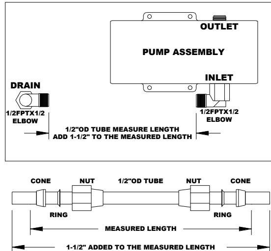
PWS APK-1 Hose Installation Diagram
