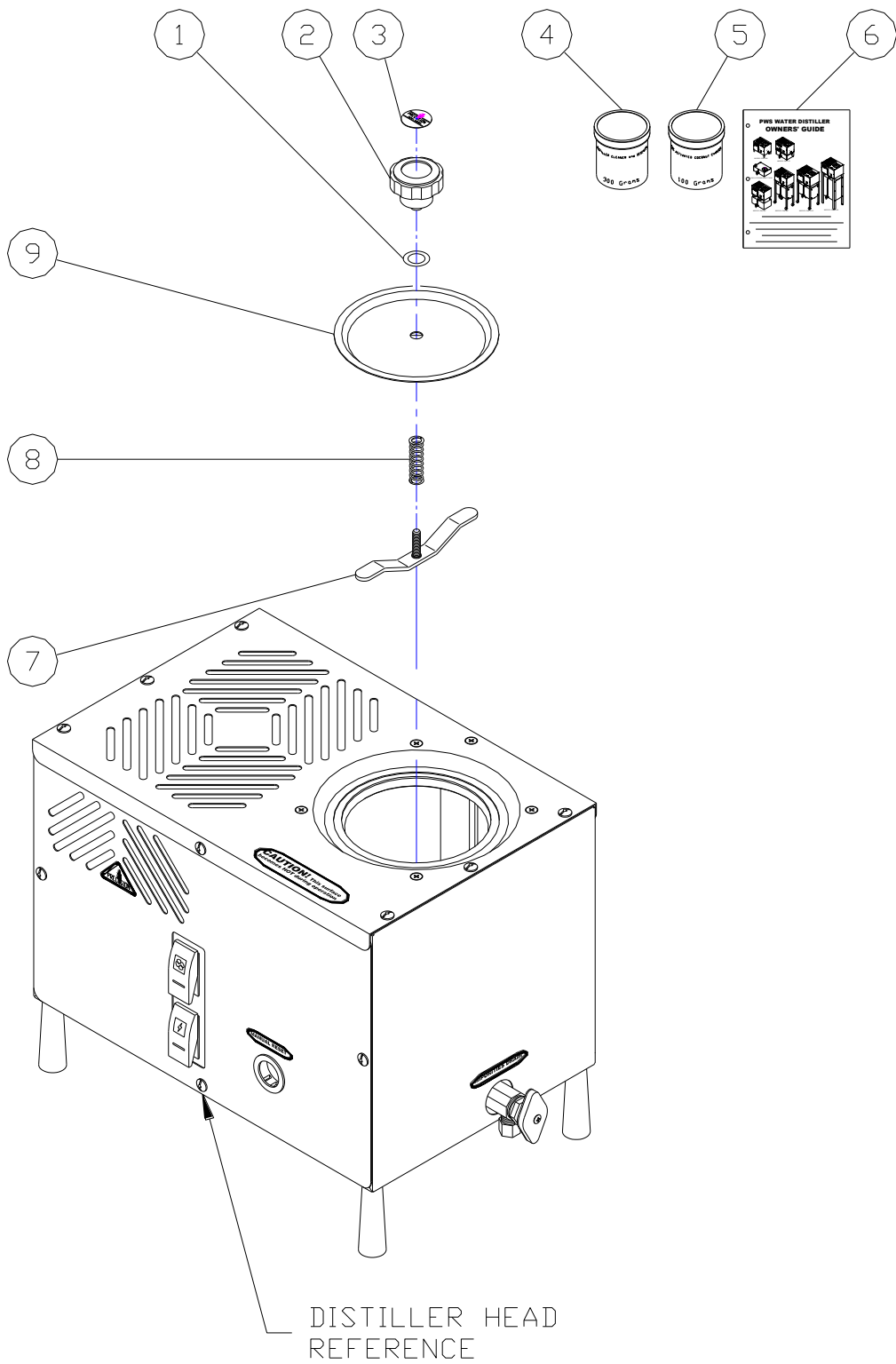
BOILING TANK LID ASSEMBLY (PART # 500184)
