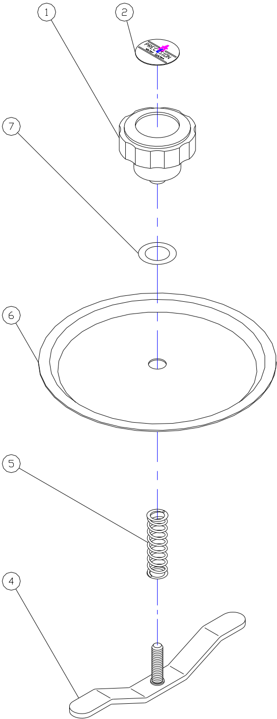
BOILING TANK LID ASSEMBLY (PART # 500184)
