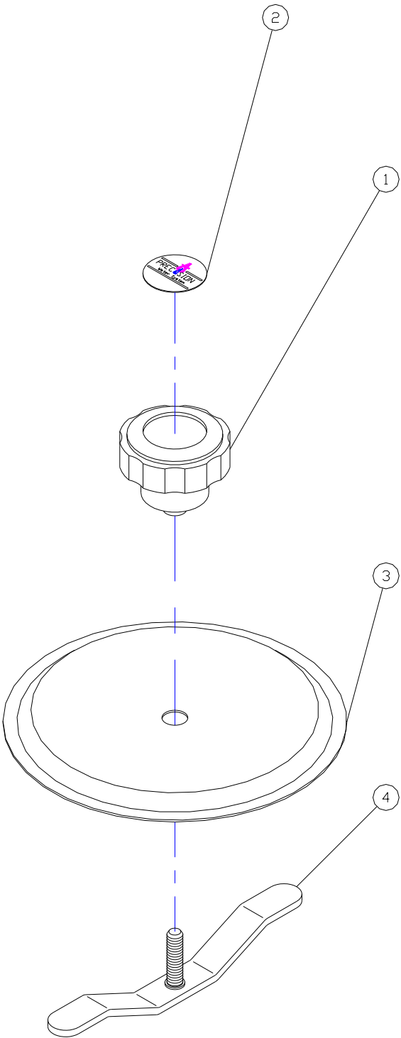
HOLDING TANK LID ASSEMBLY (PART # 500248)
