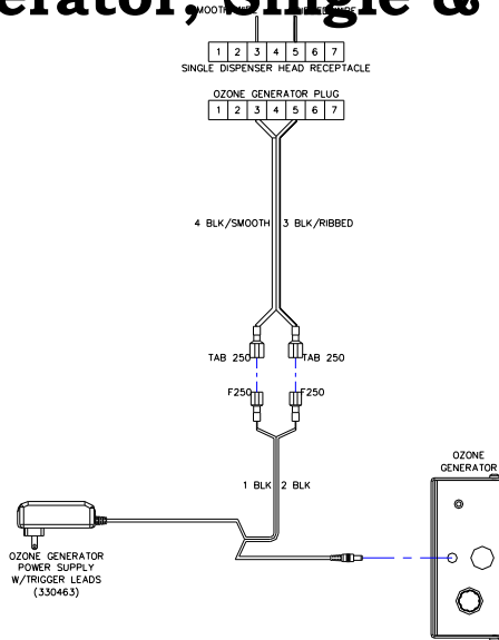
SINGLE DISPENSER OZONE GENERATOR WIRING DIAGRAM
