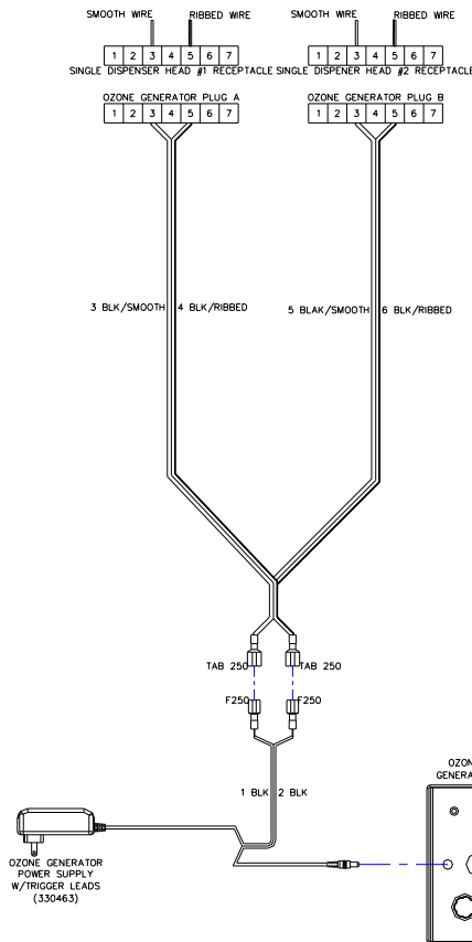
DUAL DISPENSER OZONE GENERATOR WIRING DIAGRAM
